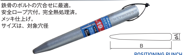
POSITIONING PUNCH
